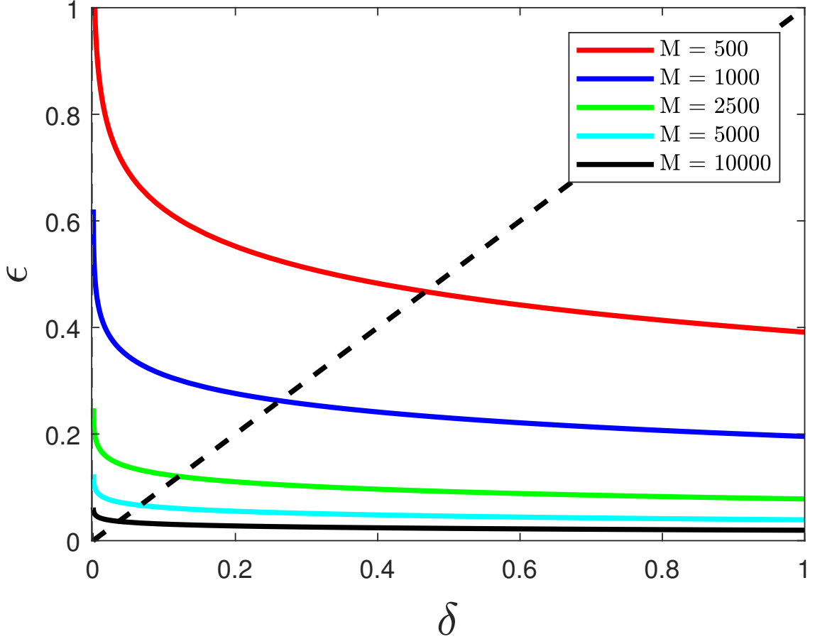
Figure 2: Iso-draw curves. At a fixed M , the combinations of \epsilon - \delta such that M = (2d/\epsilon) \ln(2d/\delta) . In this example d = 25 .
